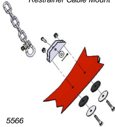
Restrainer Cable Mount
